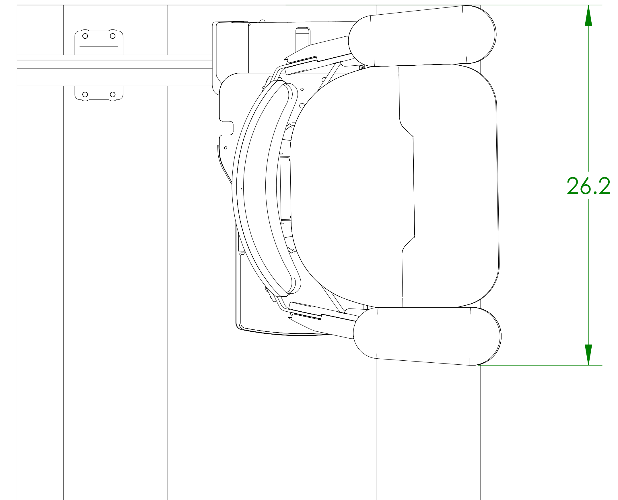
SEAT SWIVELED 90°
